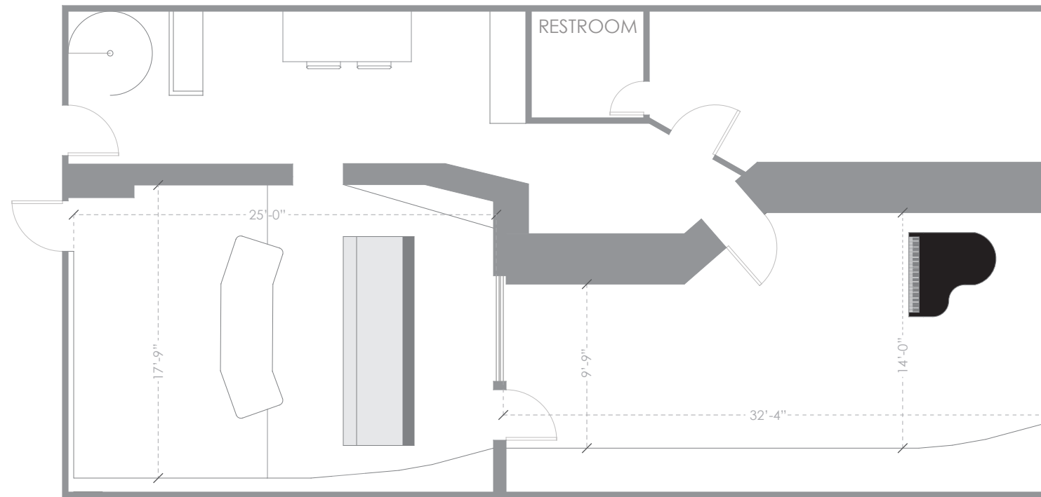
LEVEL 1 1/8" = 1'
