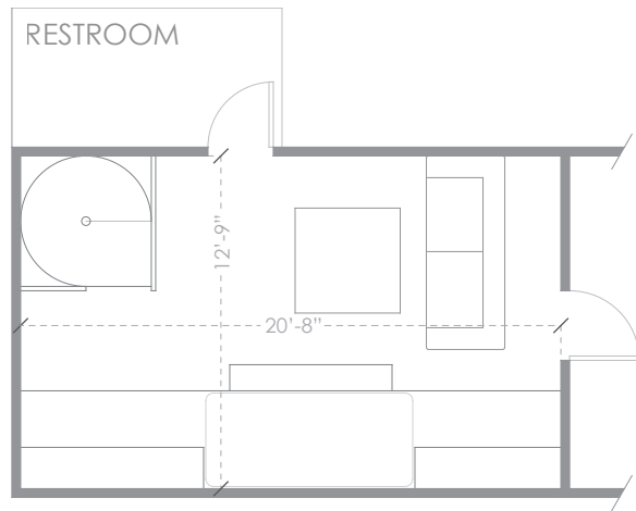
LEVEL 2 1/8" = 1'
